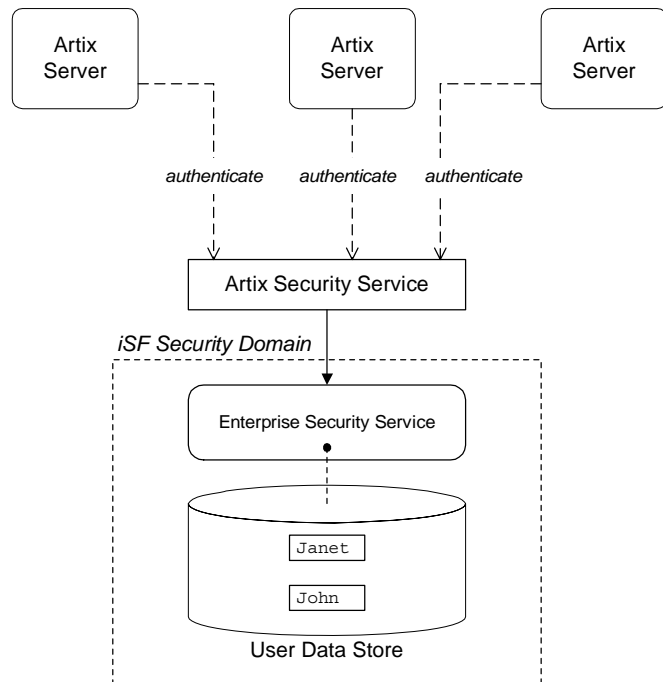
Figure 26: Architecture of an Artix security domain
