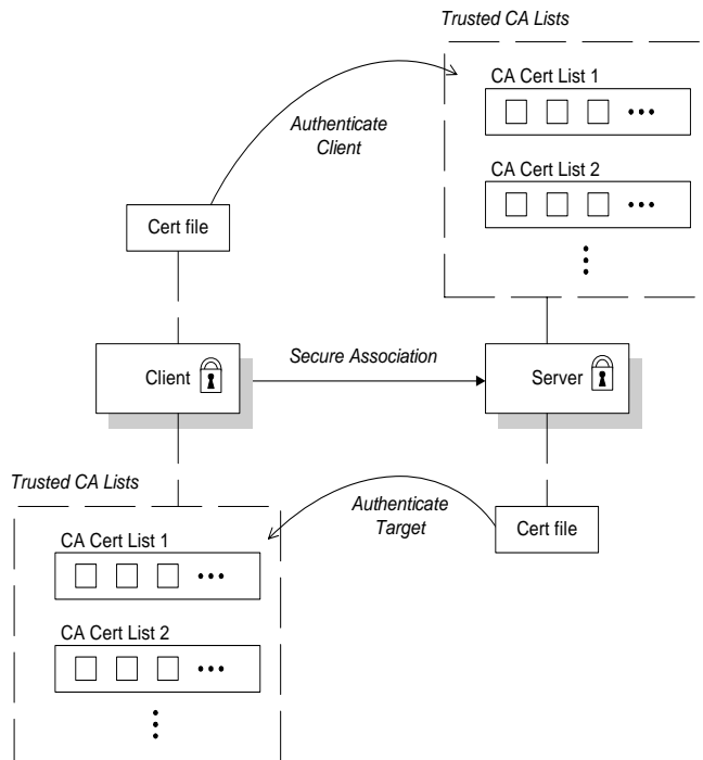
Figure 35: Mutual Authentication
