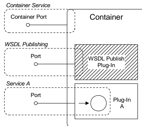
Figure 22: WSDL Publish Plug-In Deployed in a Secure Container
