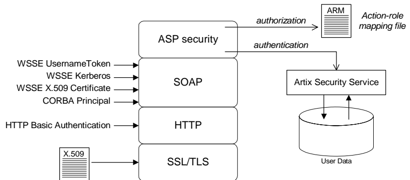
Figure 12: Overview of Security for SOAP Bindings
