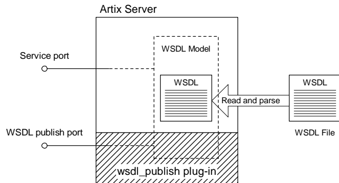
Figure 21: Endpoints Used by the WSDL Publishing Service
