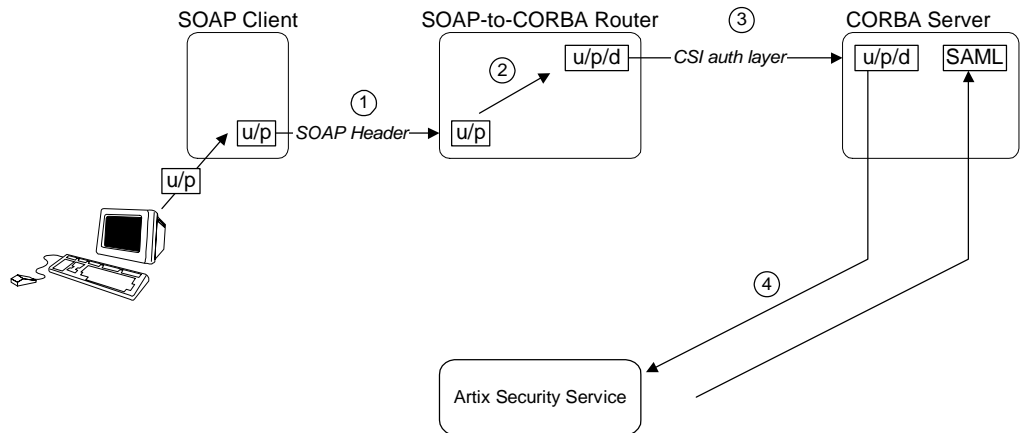
Figure 38: Propagating Credentials Across a SOAP-to-CORBA Router
