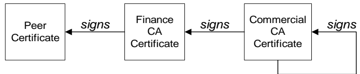
Figure 32: A Certificate Chain of Depth 3
