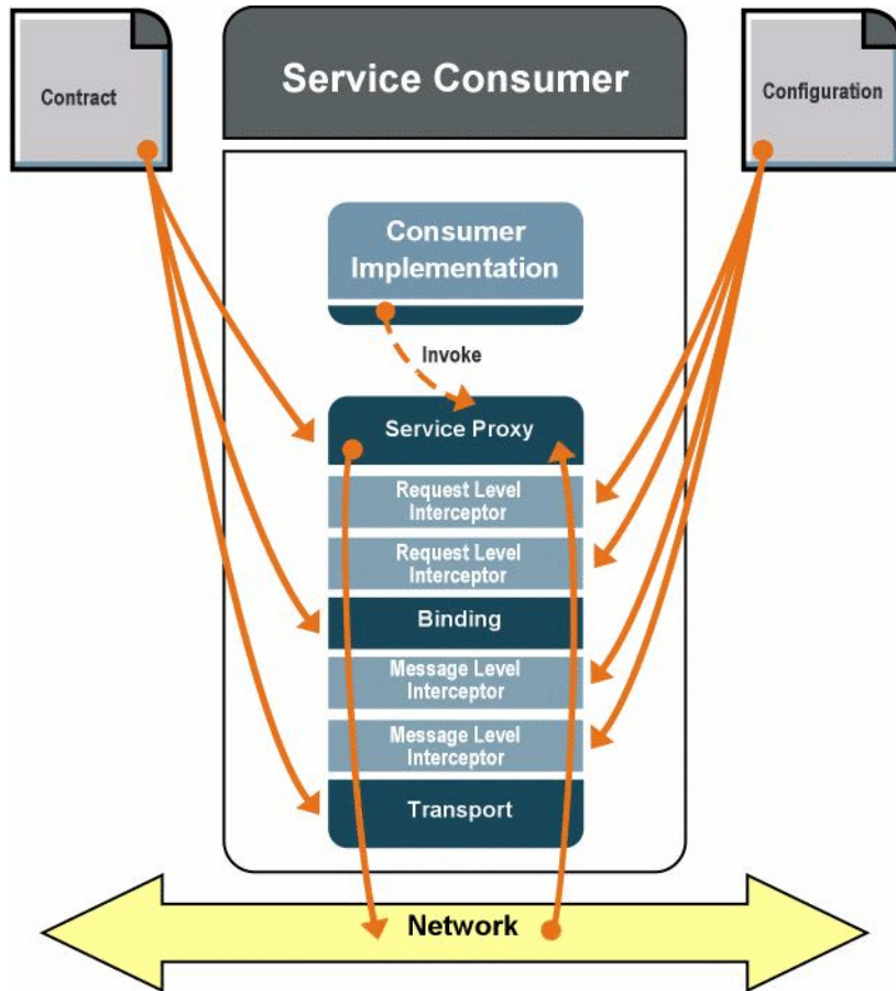
Figure 8: High-level View of a Consumer Endpoint
