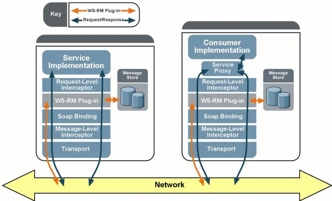
Figure 15: Overview of WS-RM Architecture
