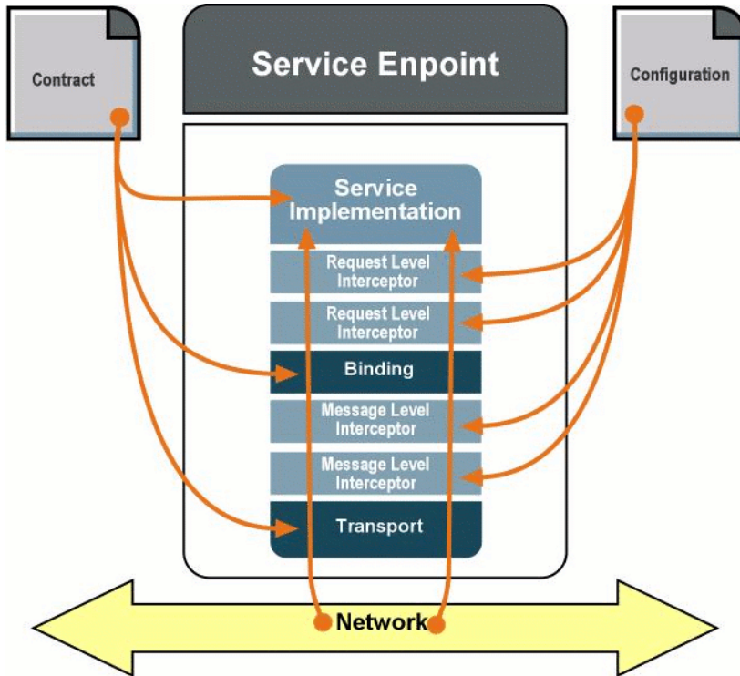
Figure 7: High-level View of a Service Endpoint
