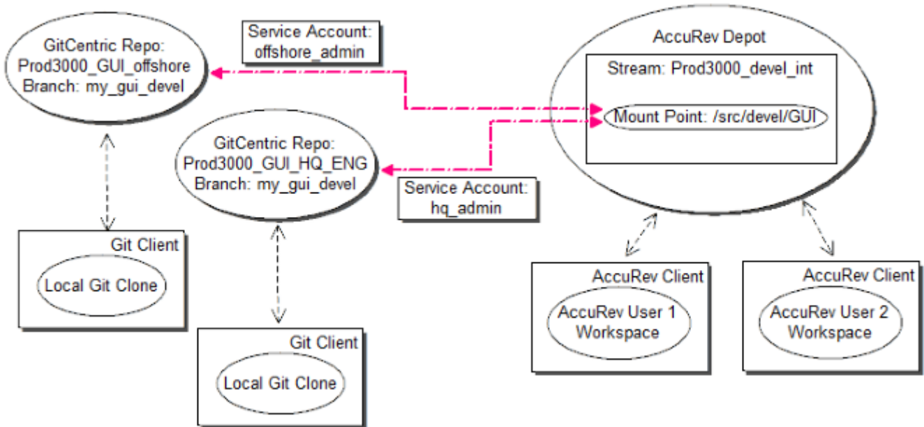
Figure 2: Security-based (same stream, same mount point, different service account)
