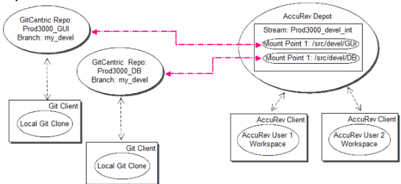
Figure 1: Project-based (same stream, different mount points)
