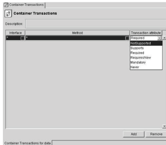
Figure 9.6 New container transaction
