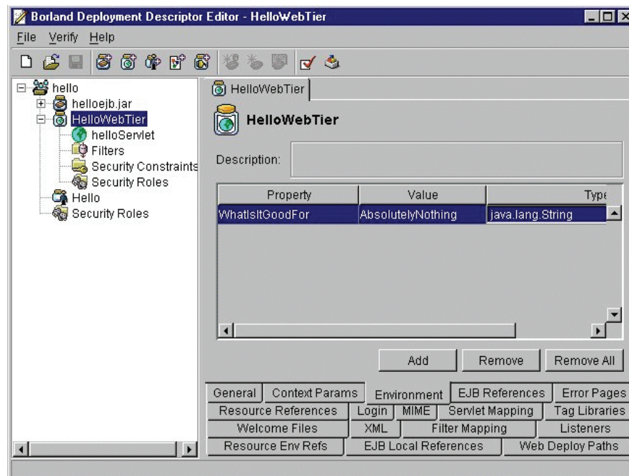
Figure 9.1 Adding an environment property
