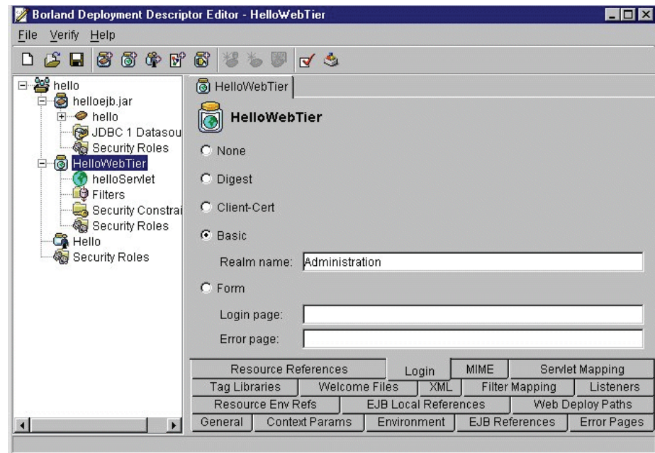
Figure 9.2 Setting login and error pages for Form-based authentication
