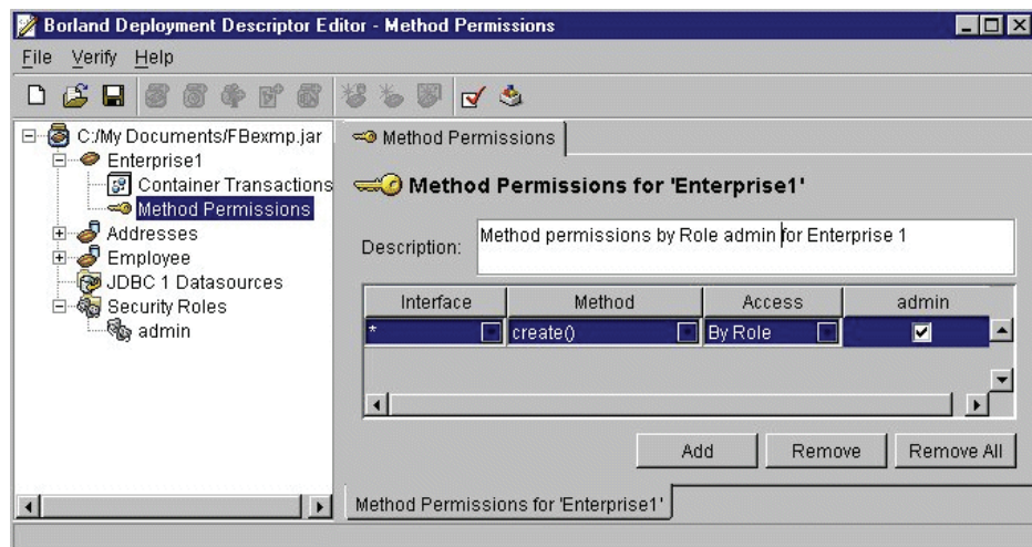
Figure 9.8 Specifying Method Permissions
