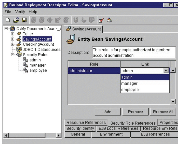
Figure 9.5 Security role references panel
