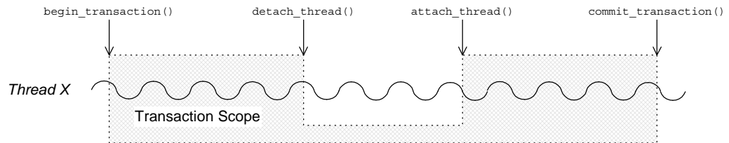
Figure 16: Detaching and Re-Attaching a Transaction to a Thread
