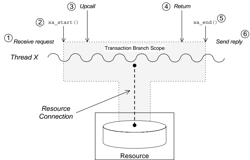
Figure 19: Auto-Association with a Single Registered Resource
