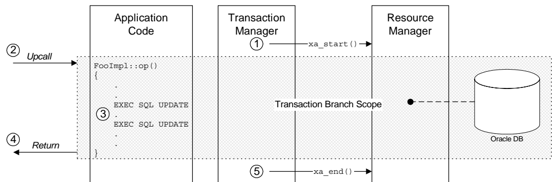
Figure 11: Invocation Dispatch for a Normally Registered RM
