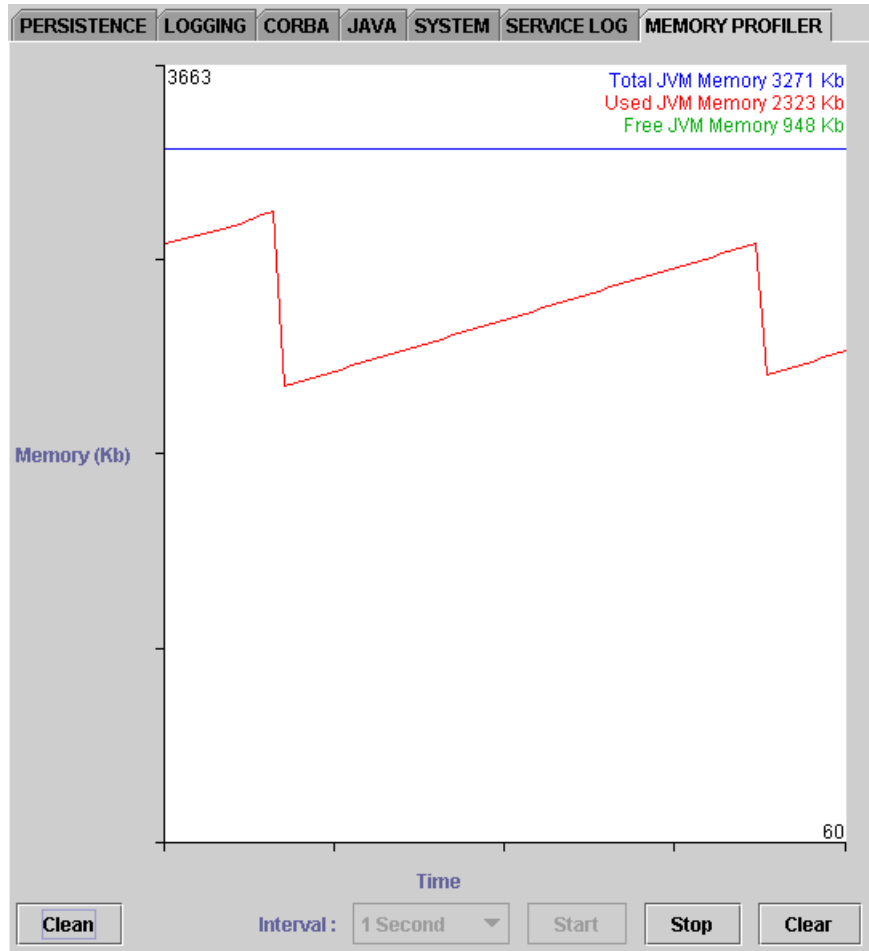
Figure 9 Memory Profiler
