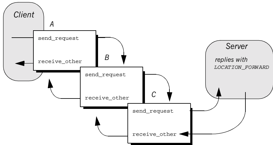
Figure 49: Client interceptors process a LOCATION_FORWARD reply.
