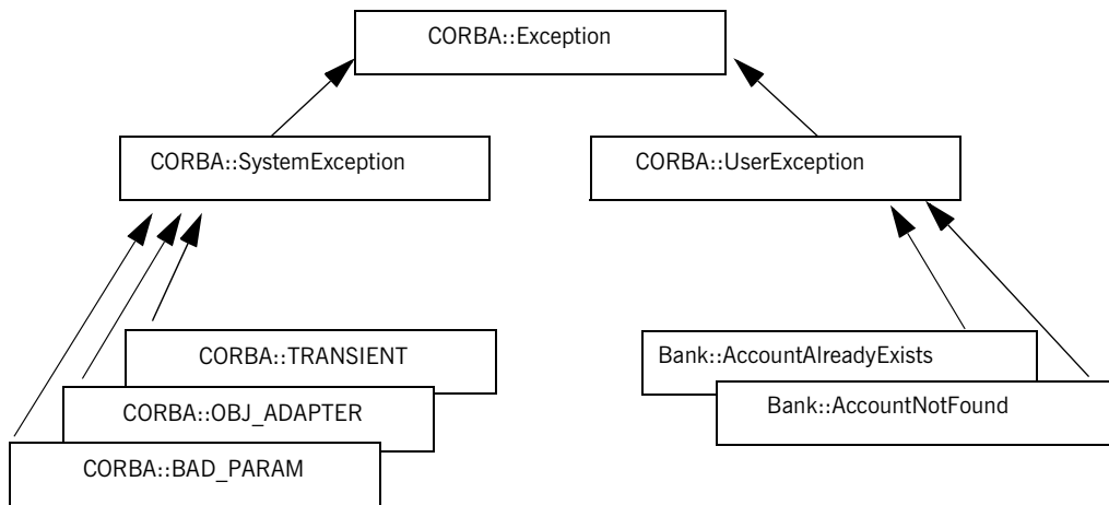
Figure 25: The C++ mapping arranges exceptions into a hierarchy
