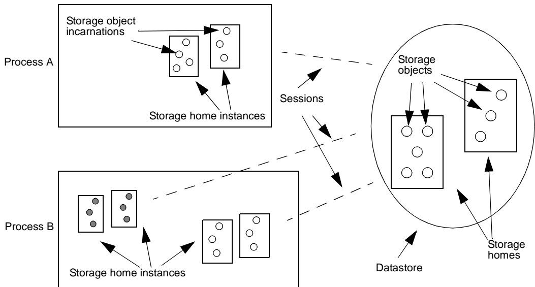
Figure 38: A server process uses sessions to establish a logical connection with a datastore and its contents
