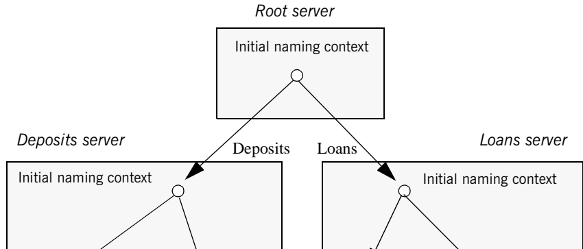
Figure 34: Multiple naming graphs are linked by binding initial naming contexts of several servers to a root server.
