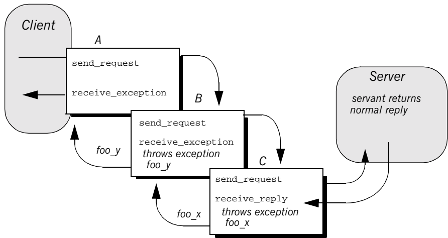
Figure 51: Client interceptors can change the nature of the reply.
