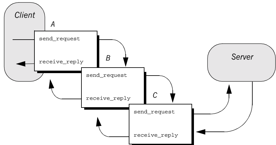
Figure 48: Client interceptors process a normal reply.
