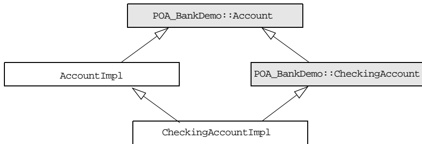
Figure 18: A servant class can inherit base class implementations.
