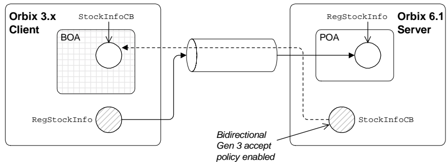
Figure 57: Orbix 3 Client Receiving a Callback from an Orbix 6.1 Server
