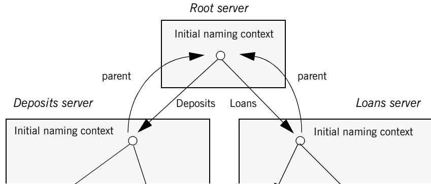
Figure 35: The root server's initial naming context is bound to the initial naming contexts of other servers, allowing clients to locate the root naming context.
