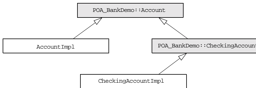
Figure 19: A servant class can implement operations of all base skeleton classes.
