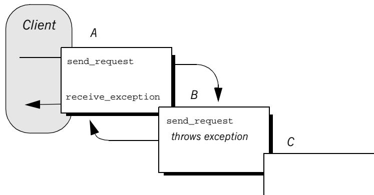
Figure 50: send_request throws an exception in a client-side interceptor
