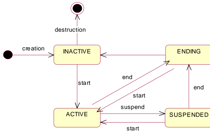
Figure 39: Transactional session states
