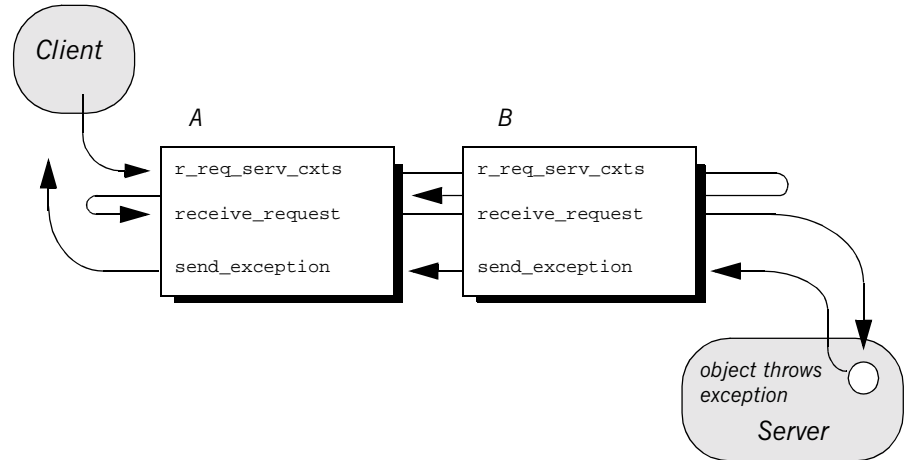
Figure 52: Server interceptors receive request and send exception thrown by target object.
