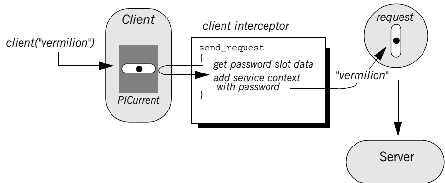
Figure 47: PICurrent facilitates transfer of thread context data to a request or reply.
