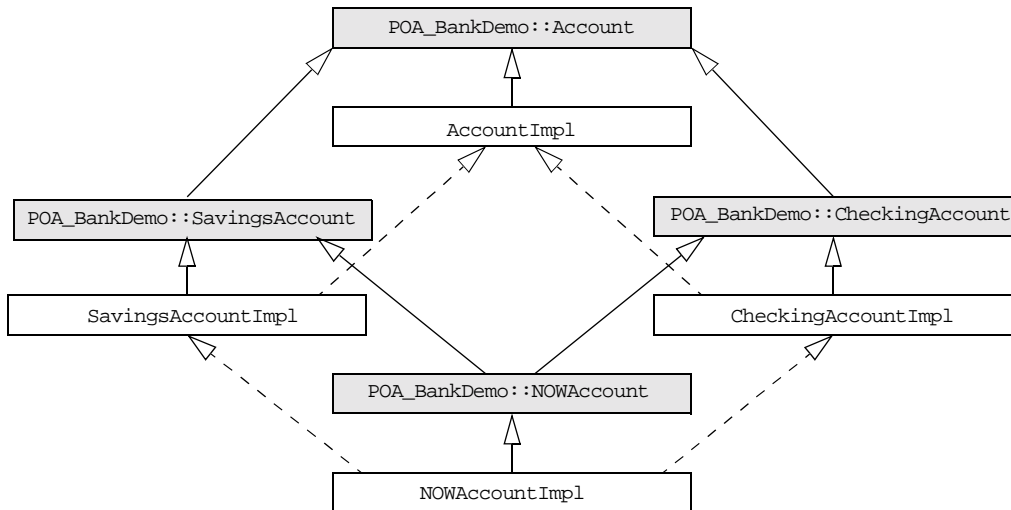
Figure 20: Inheritance options among servant and base skeleton classes.
