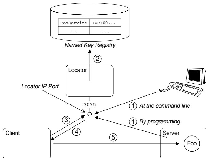
Figure 58: Using corbaloc with the Locator-Based Named Key Registry
