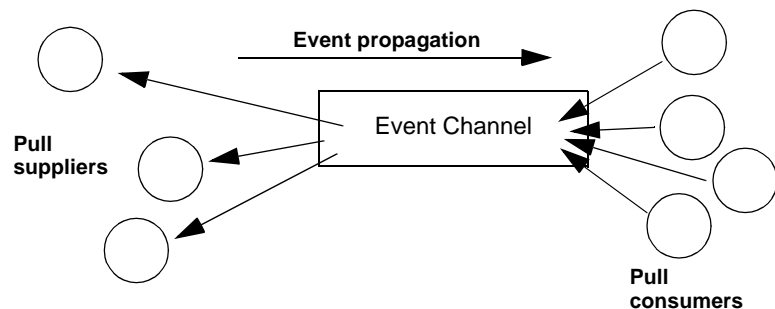
Figure 43: Pull Model suppliers and consumers communicating through an event channel
