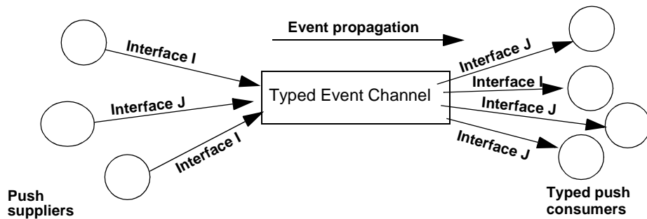
Figure 45: Push consumers pushing typed events to typed push consumers
