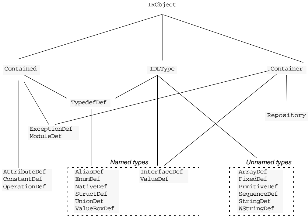
Figure 27: Hierarchy of interface repository objects
