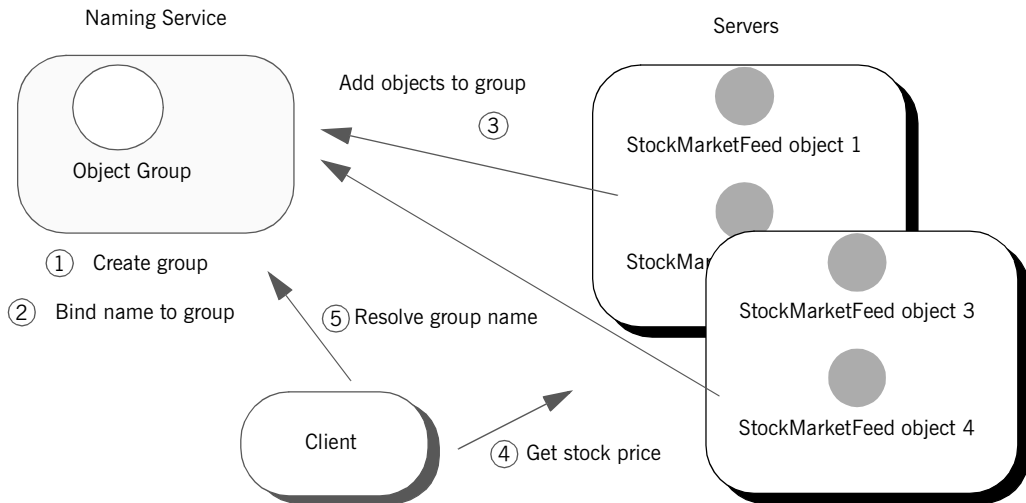
Figure 37: Architecture of the stock market example
