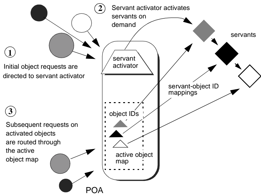
Figure 22: On the first request on an object, the servant activator returns a servant to the POA, which establishes the mapping in its active object map.
