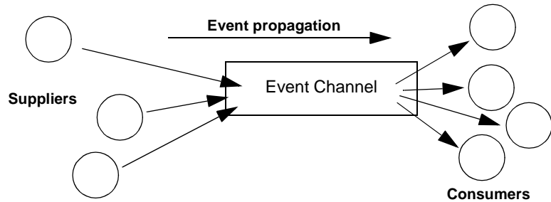
Figure 40: Suppliers and consumers communicating through an event channel
