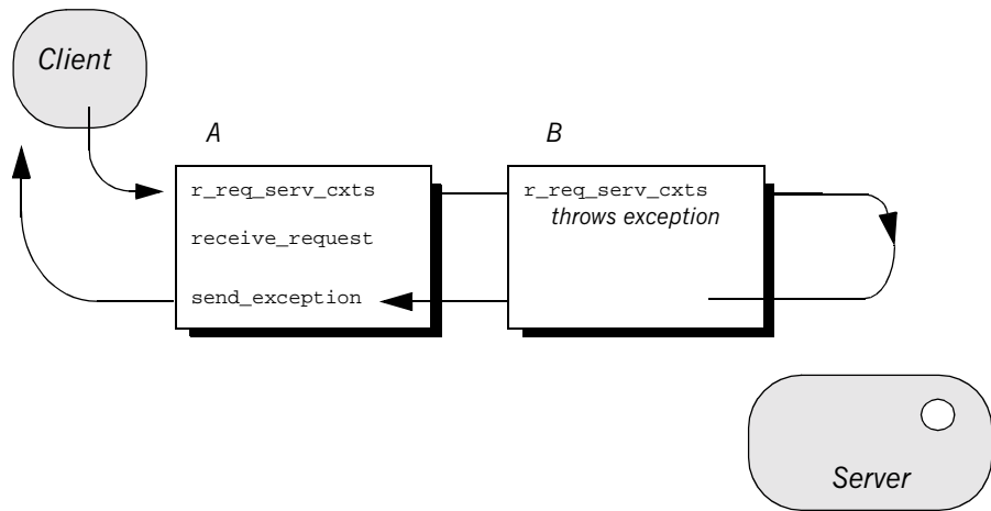
Figure 53: receive_request_service_contexts throws an exception and interception flow is aborted.
