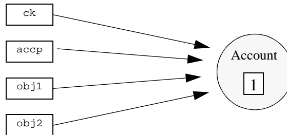
Figure 16: Multiple _ptr references to a proxy object can leave the reference count unchanged.
