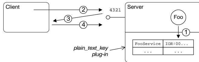
Figure 59: Using corbaloc with the plain_text_key Plug-In
