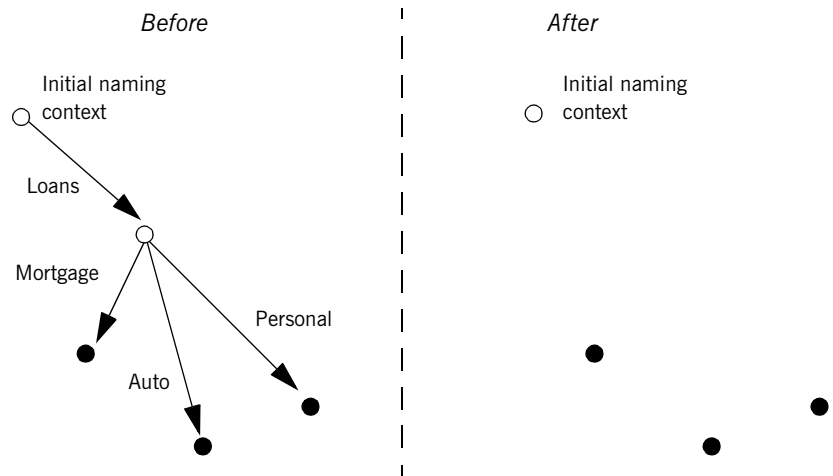
Figure 32: Destroying a naming context and removing related bindings
