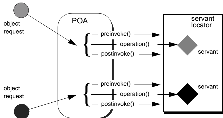
Figure 23: The POA directs each object request to the servant locator, which returns a servant to the POA to process the request.
