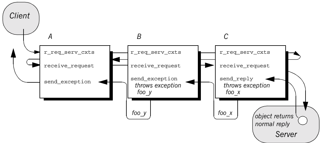
Figure 54: Server interceptors can change the reply type.
