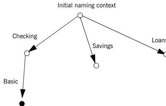
Figure 31: Binding an object reference to a naming context
