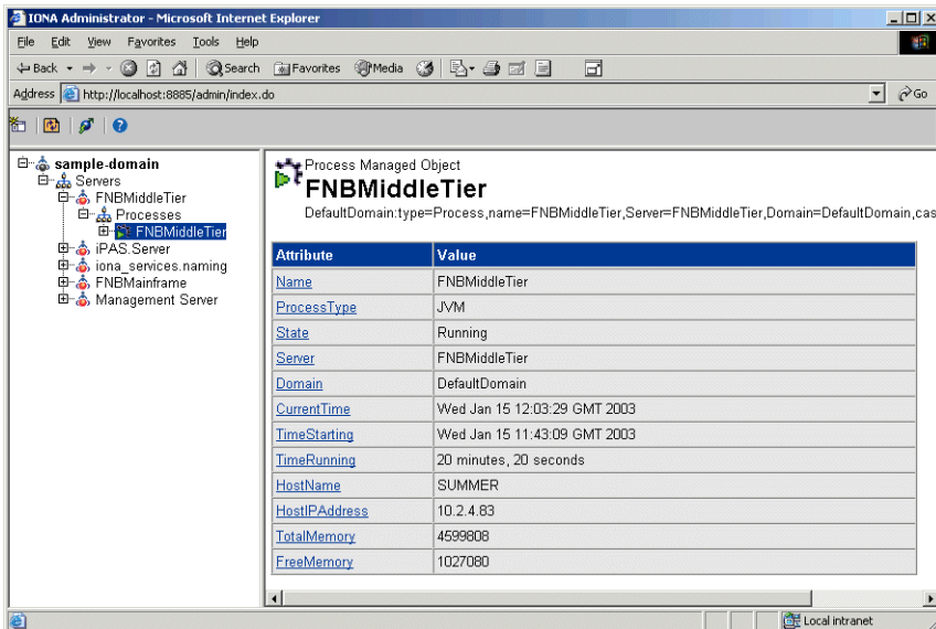
Figure 8: FNBMiddleTier Process MBean
