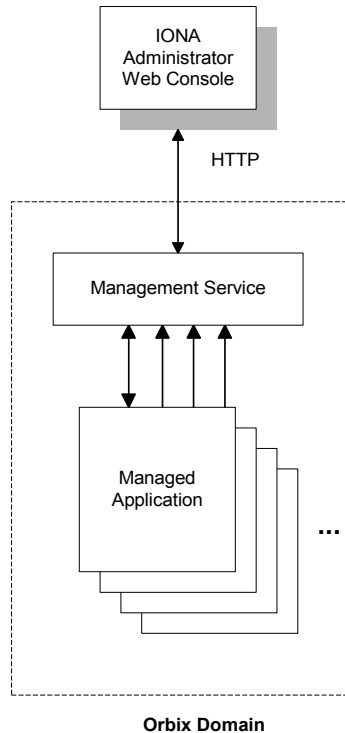
Figure 1: IONA Administrator Components
