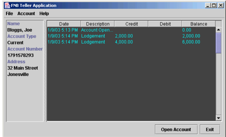
Figure 4: FNB Teller Application
