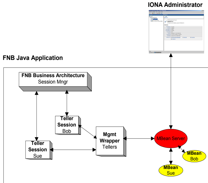
Figure 6: FNB Application Overview
