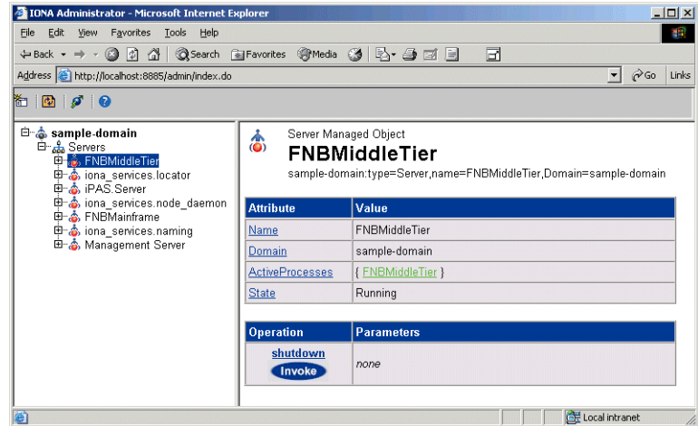
Figure 5: FNB Displayed in IONA Administrator
