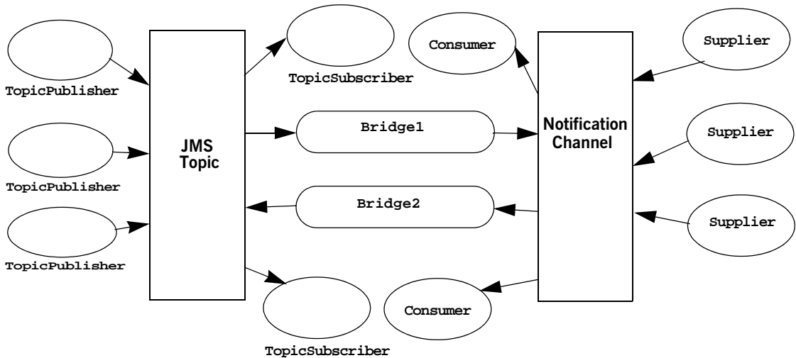
Figure 7: JMS-Notification Bridging
