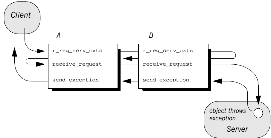
Figure 57: Server interceptors receive request and send exception thrown by target object.
