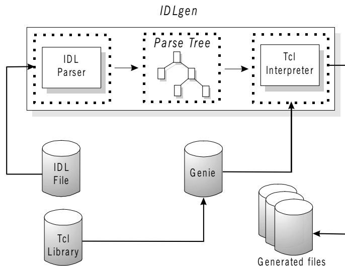
Figure 2: Code Generation Toolkit Components
