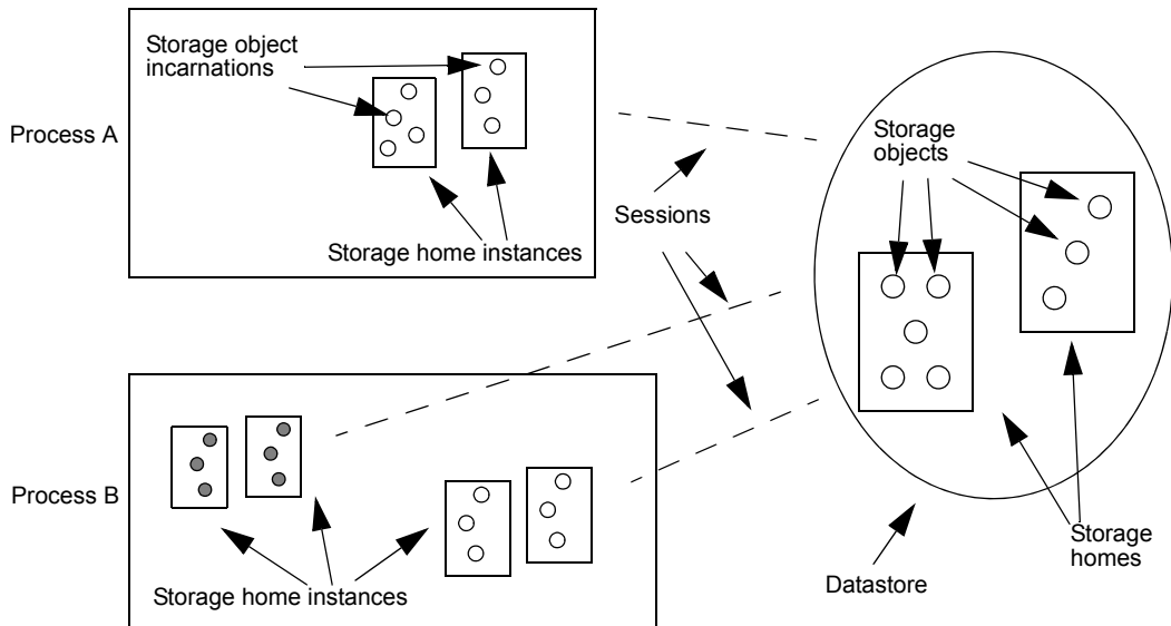
Figure 40: A server process uses sessions to establish a logical connection with a datastore and its contents
