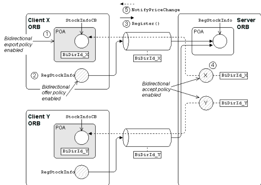
Figure 60: Basic Bidirectional GIOP Scenario—Stock Feed
