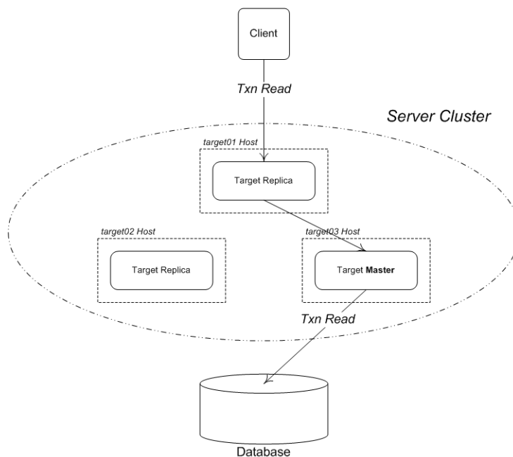
Figure 43: Delegation Required for Transactional Read Operation
