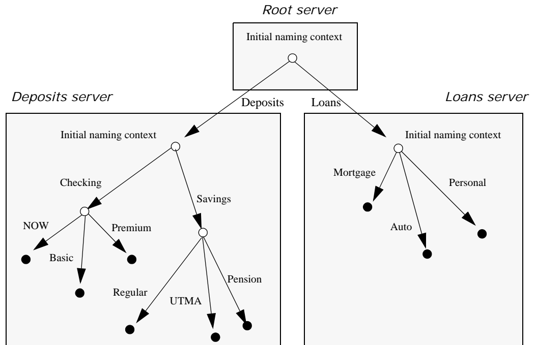
Figure 28: A naming graph that spans multiple servers
