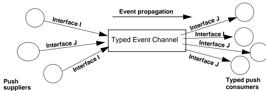
Figure 38: Push consumers pushing typed events to typed push consumers
