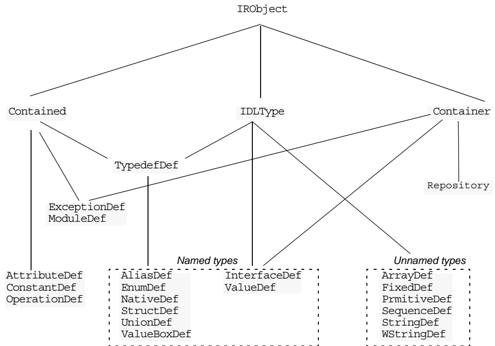
Figure 22: Hierarchy of interface repository objects
