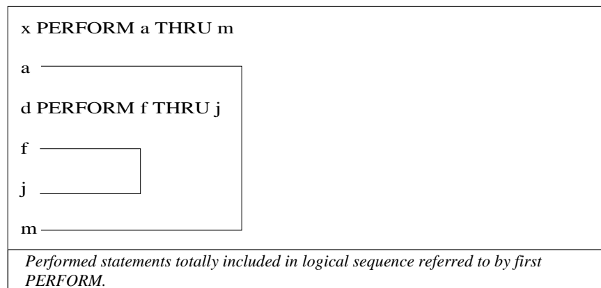
Figure 9: PERFORM Statement Examples
