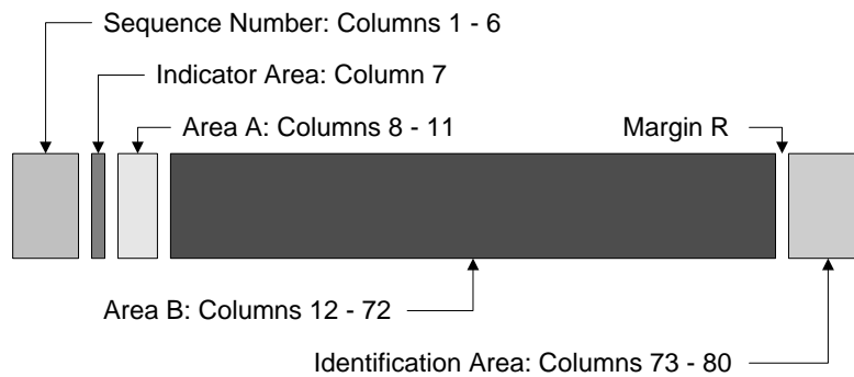
Figure 2: Example of Traditional Source Format
