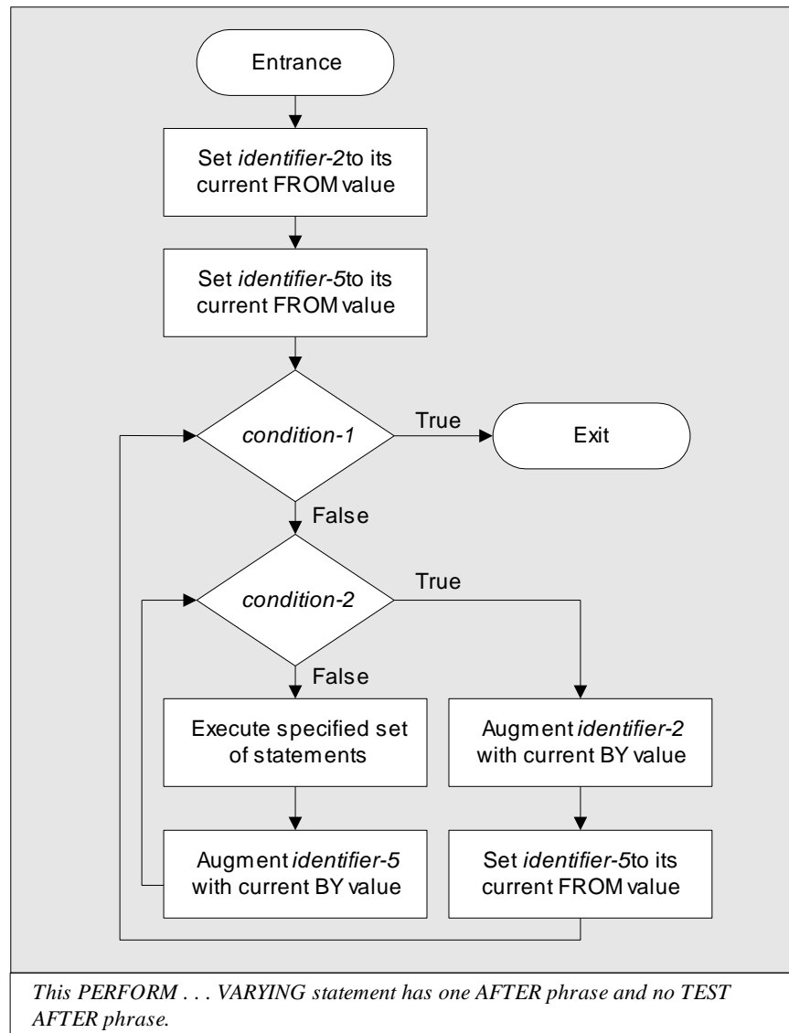
Figure 6: PERFORM . . . VARYING Statement
