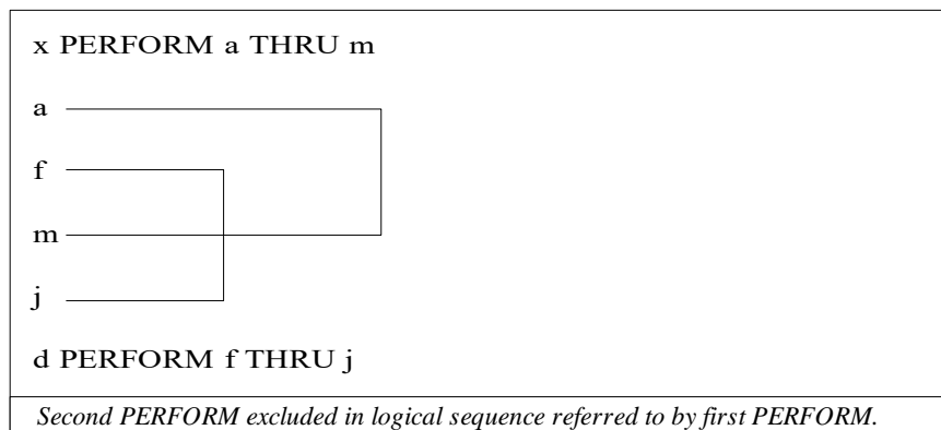
Figure 11: PERFORM Statement Examples
