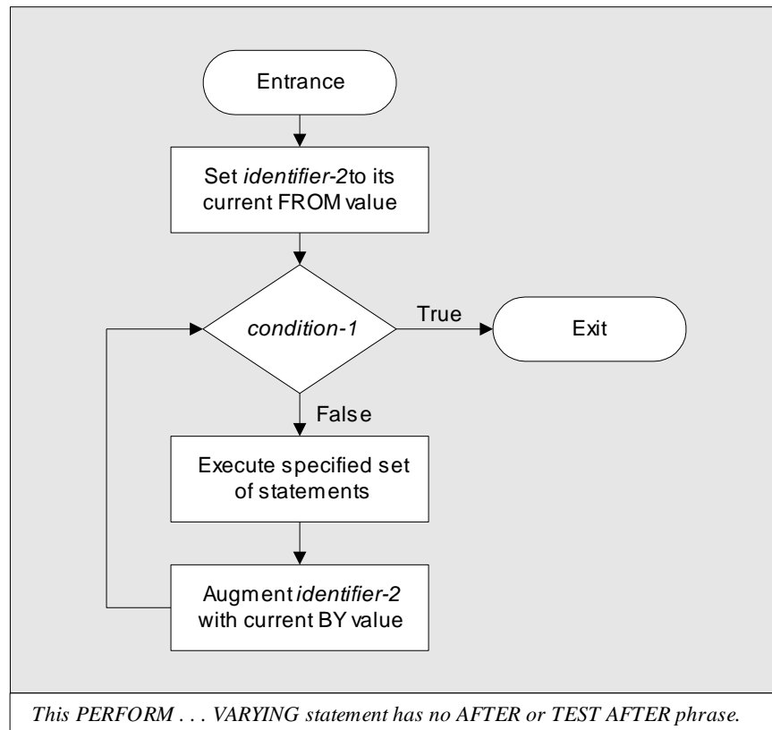
Figure 5: PERFORM . . . VARYING Statement
