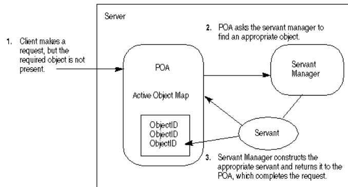
Figure 7 Example servant manager function
