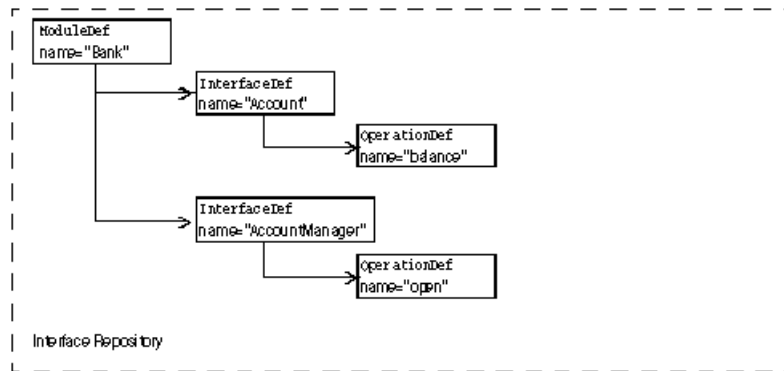
Figure 31 Interface repository object hierarchy for Bank.idl
