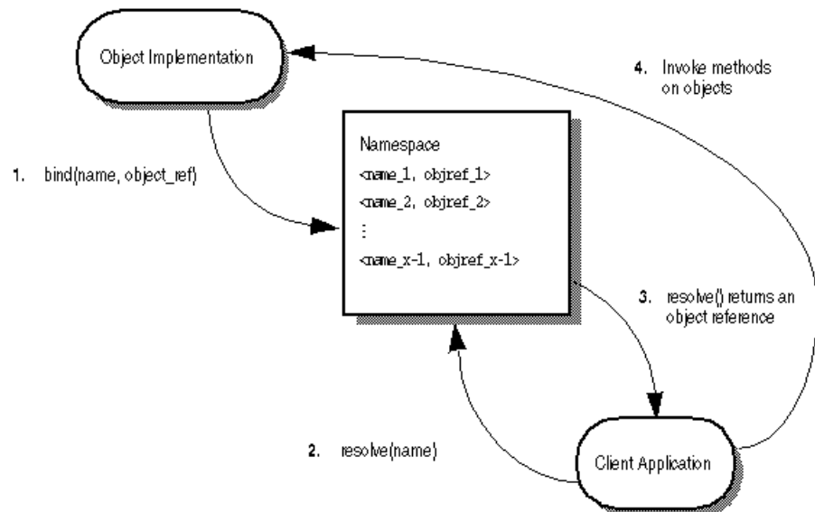
Figure 25 Binding, resolving, and using an object name from a naming context within a namespace
