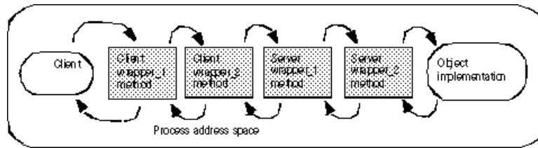
Figure 38 Typed object wrapper invocation order
