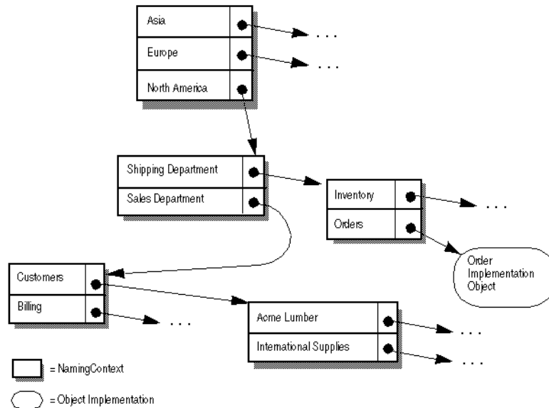
Figure 26 Naming scheme for an order entry system
