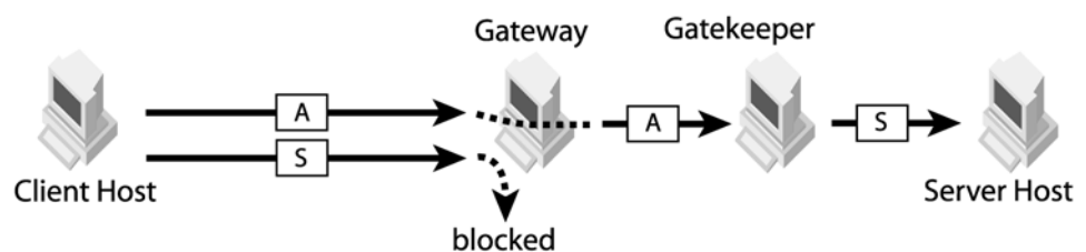
Figure 3 GateKeeper in a server network
