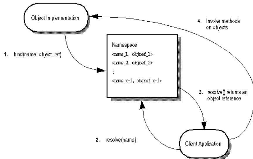
Figure 24 Binding, resolving, and using an object name from a naming context within a namespace
