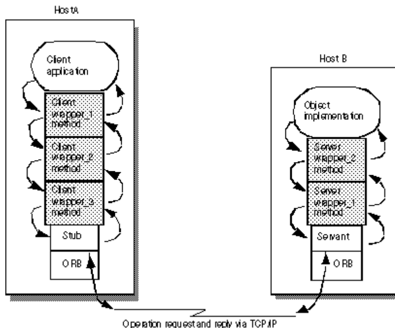
Figure 37 Multiple, typed object wrappers registered
