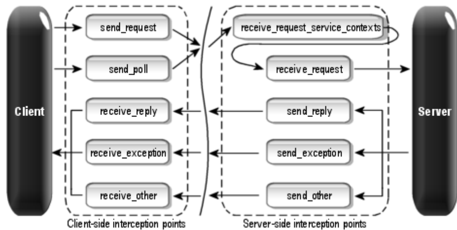
Figure 33 Request Interception points
