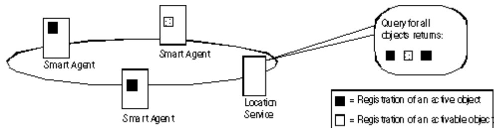
Figure 21 Using the Smart Agent to find instances of objects
