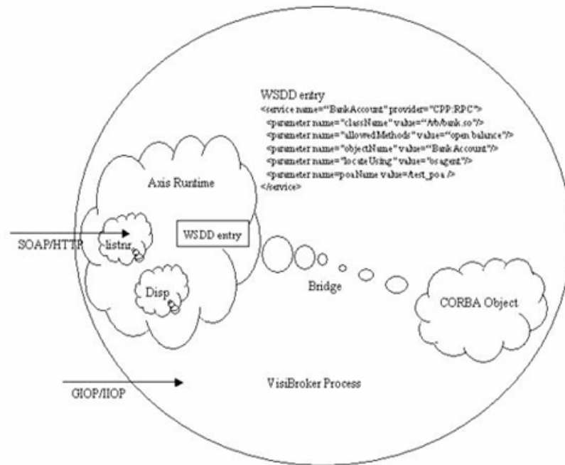
Figure 43 Components inside a VisiBroker process
