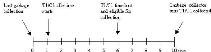
Figure 16 Collection of resources by ORB GC
