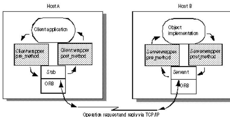
Figure 34 Single untyped object wrapper
