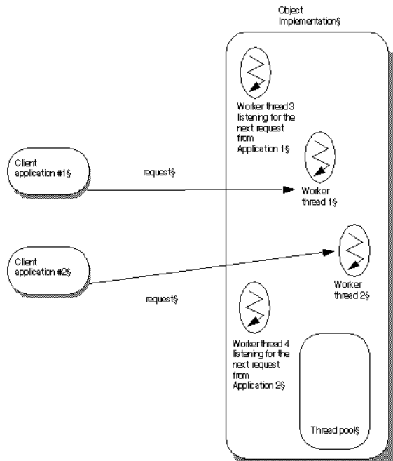
Figure 10 Client application #2 sends a request
