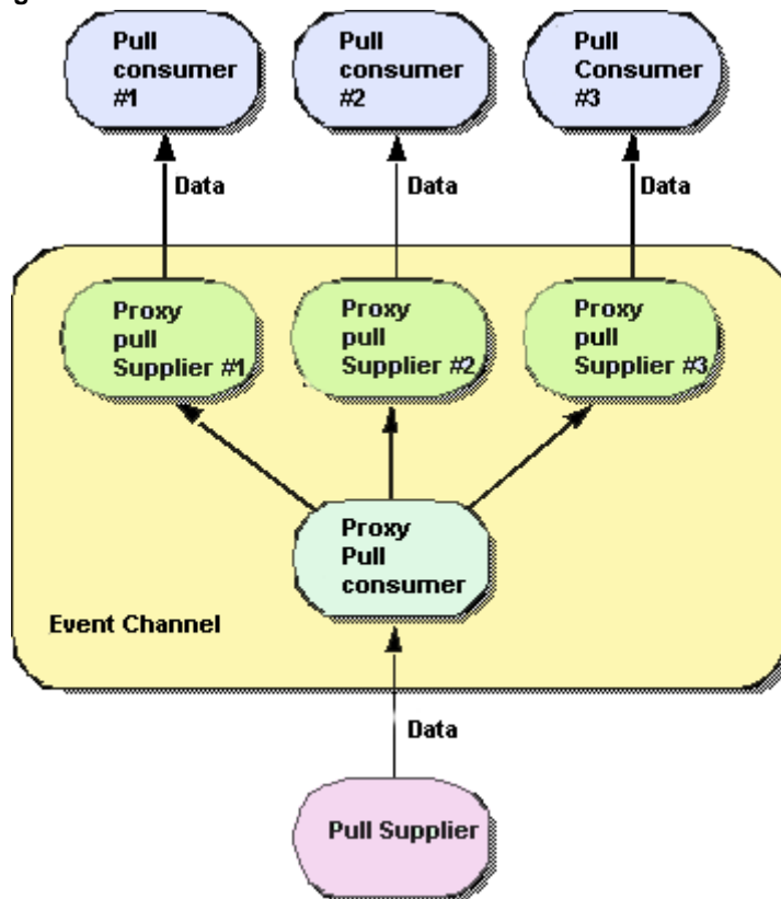
Figure 30 Pull model
