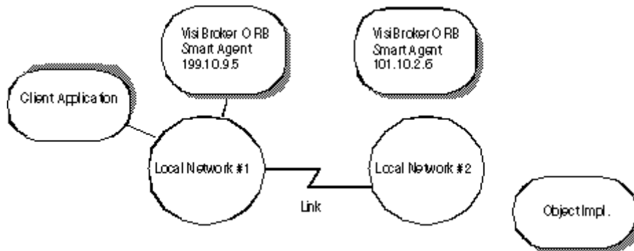
Figure 19 Two Smart Agents on separate local networks
