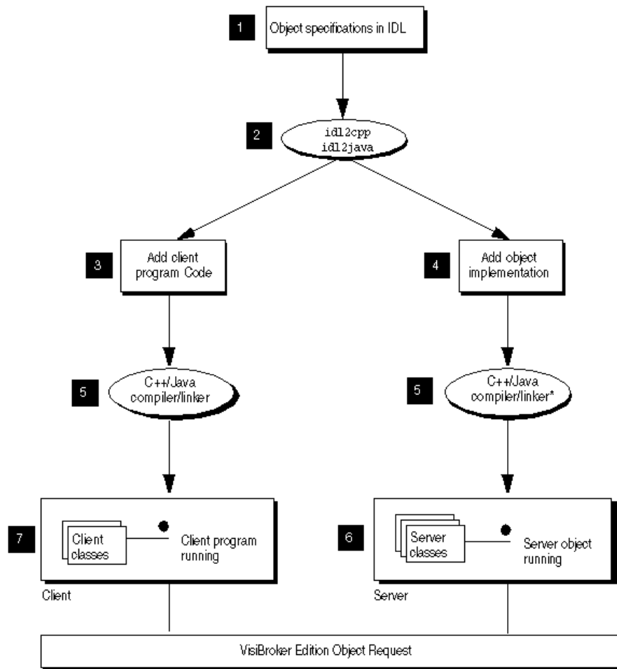
Figure 3 Developing the sample bank application
