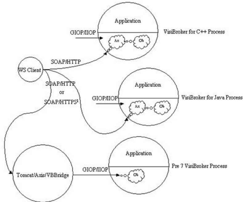
Figure 42 Web Services run-time behavior
