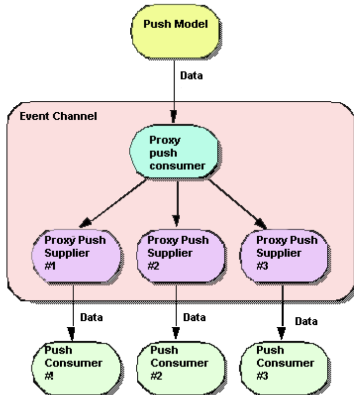
Figure 29 Push model
