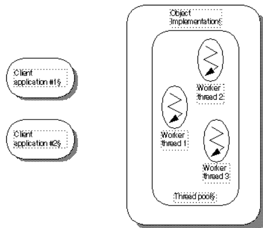
Figure 8 Pool of threads is available
