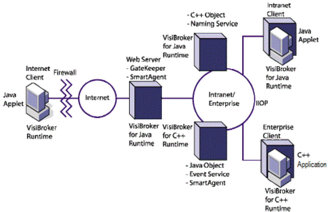
Figure 2 VisiBroker Architecture
