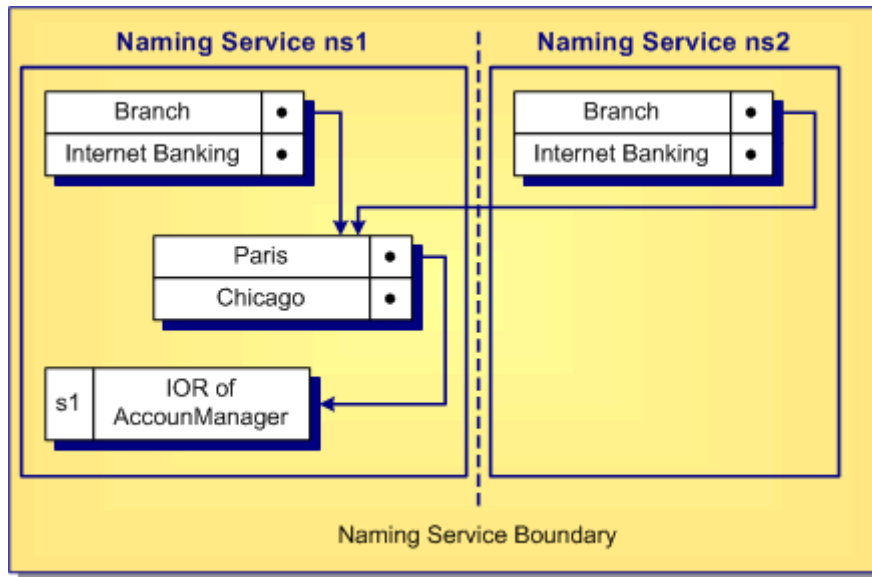
Figure 26 Naming contexts with multiple access hierarchies
