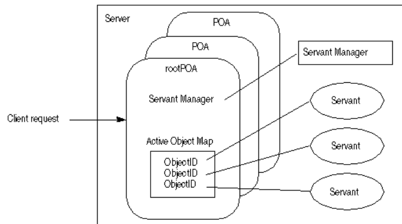
Figure 5 Overview of the POA
